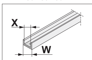
Gasket for frame profiles TYPE II S01/S02/S04
